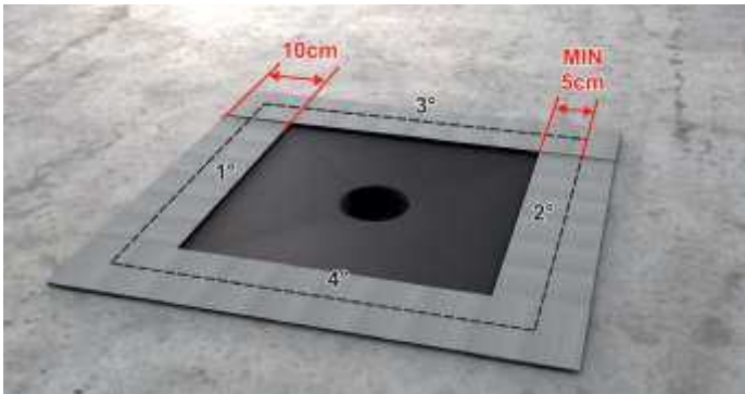
Example of installation of Bonomini's ADHESIVE waterproofing layer Art. 6822AD--C
