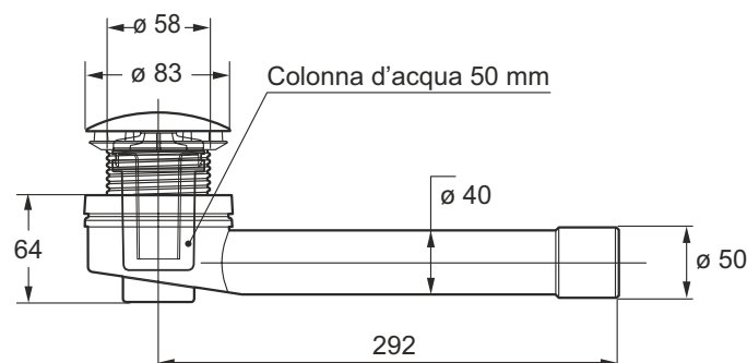
Extremely reduced height: only 64 mm below the shower tray compliant to EN-274: 50 mm water seal trap
